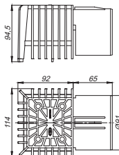
Attika-Laubfangkorb
