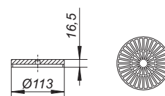
Flachrost S 10
